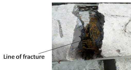
b: 1-fabric layer reinforced cement composite beam.
